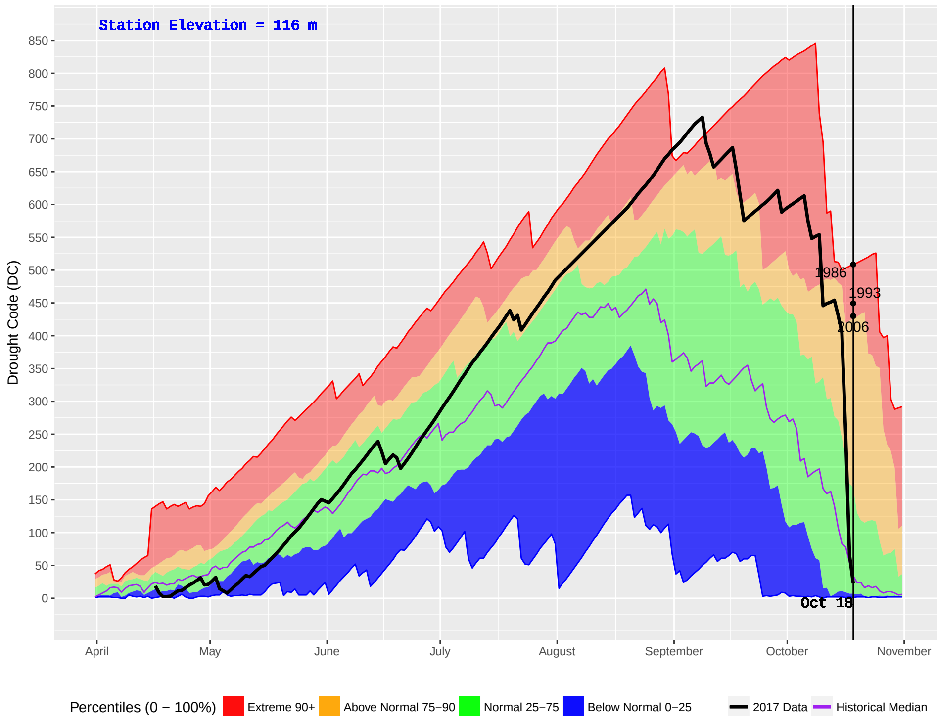
SCAR CREEK (82) : Historical (1982–2016) and Current (2017) Noon Drought Code (DC)
